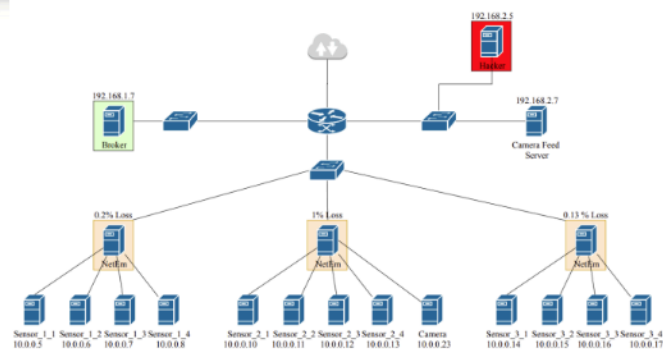
Figure 1: MQTT Network Architecture.
